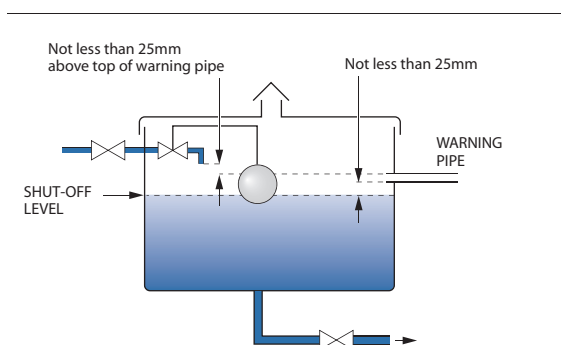
Fig. 10c: Cistern for Fluid Category 1 & 2, 1000L capacity or less (15mm (1/2") & 22mm (3/4") supplies only).
