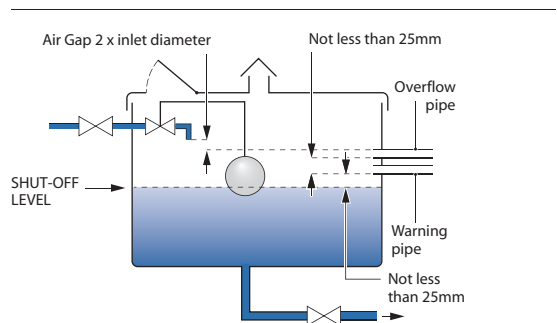
Fig. 11c: Cistern capacity 1000 L to 5000 L - Type 'AG' and 'AF' air gaps
