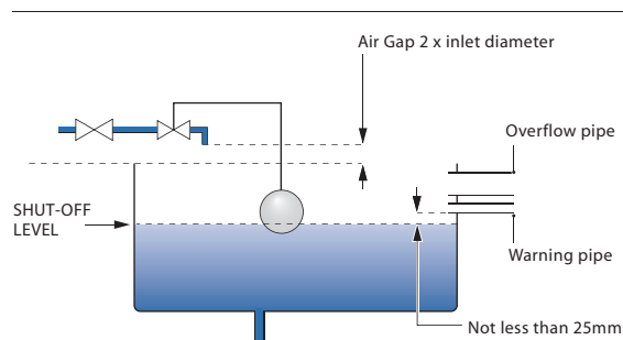
Fig. 12a: Open top cistern with an 'unrestricted' type AA' air gap.
