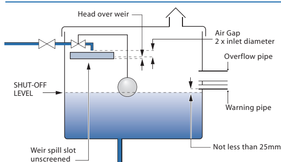
Fig. 12b: Closed top cistern – Type AB' air gap.
