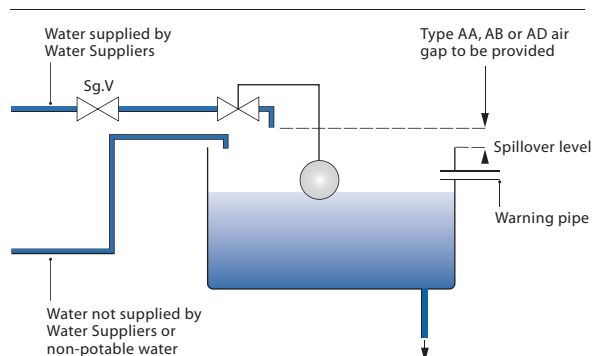
Fig. 12d: Cistern supplied with a mains supply and an alternative source.
