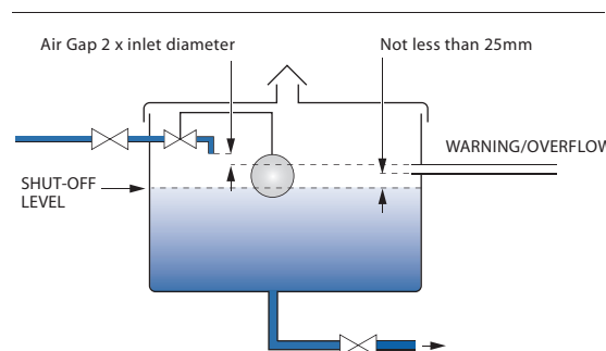
Fig. 11b: Cistern capacity 1000 L or less - Type 'AG' and 'AF'
